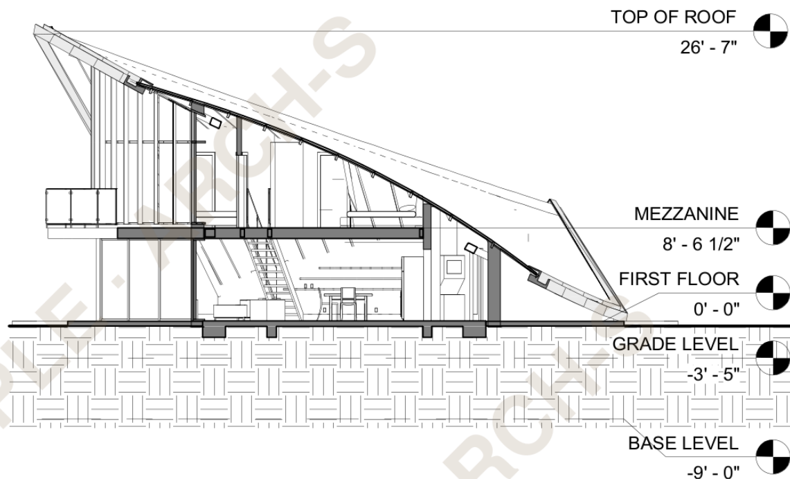
1 SECTION 1 1" = 10'-0"
